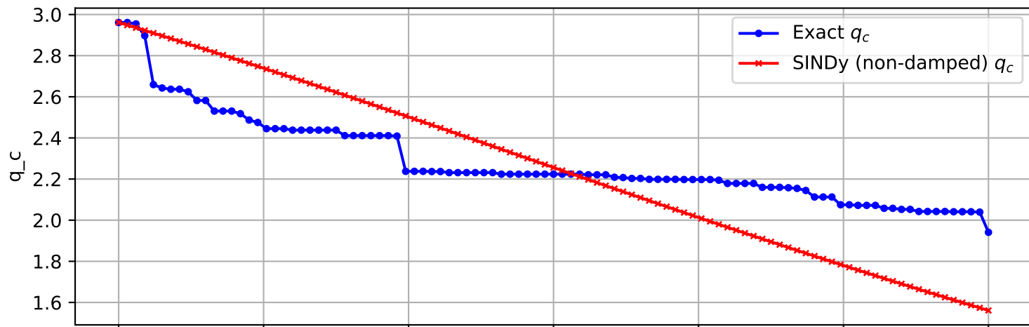
Trajectory 2664 (non-damped)
