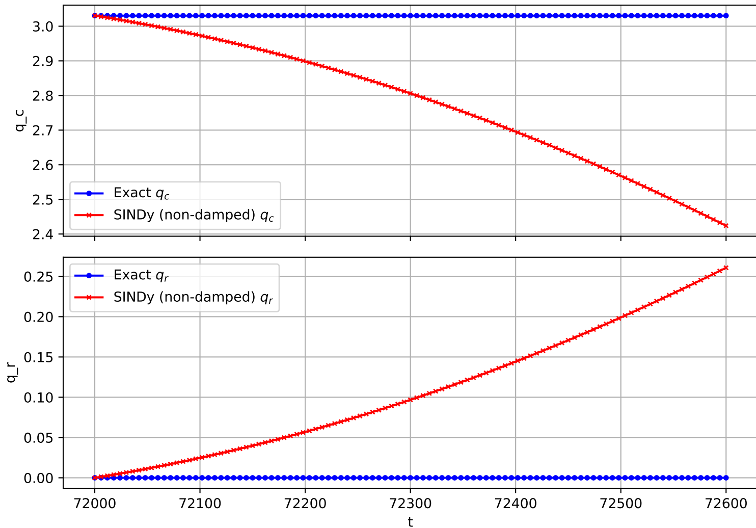
Trajectory 2672 (non-damped)
