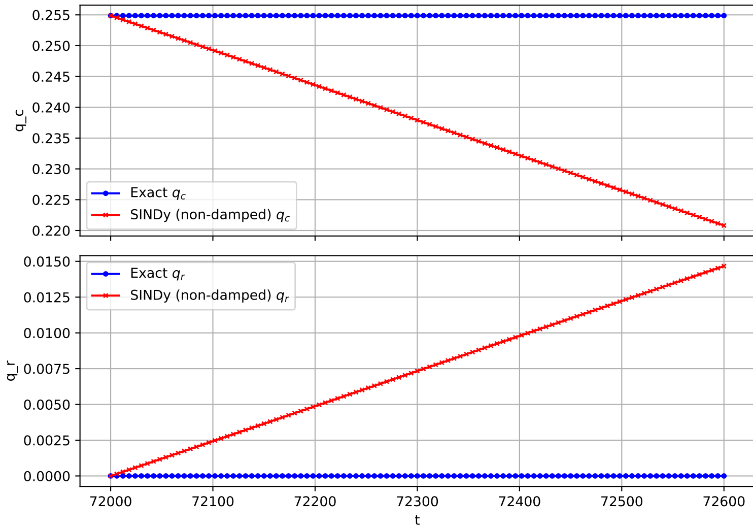
Trajectory 2673 (non-damped)
