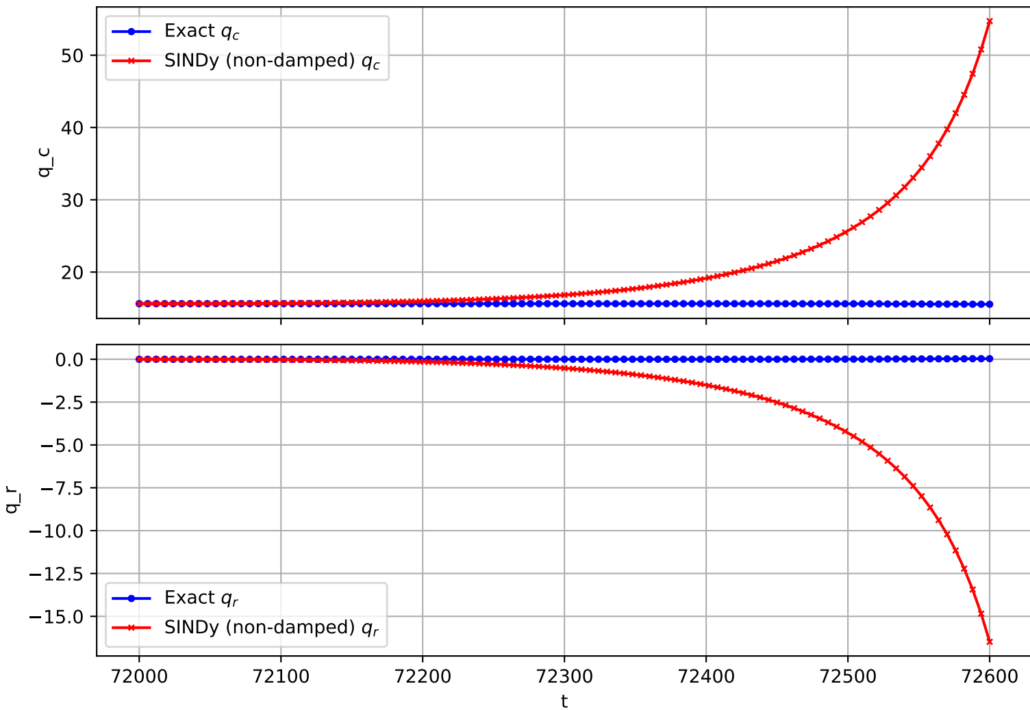
Trajectory 2676 (non-damped)
