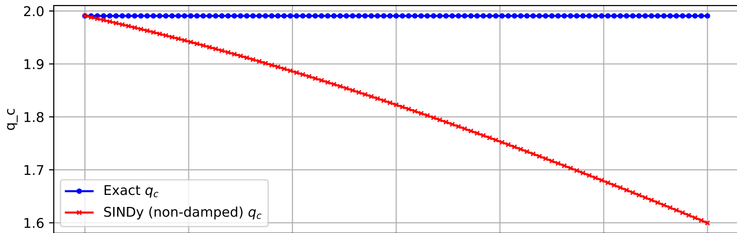
Trajectory 2682 (non-damped)
