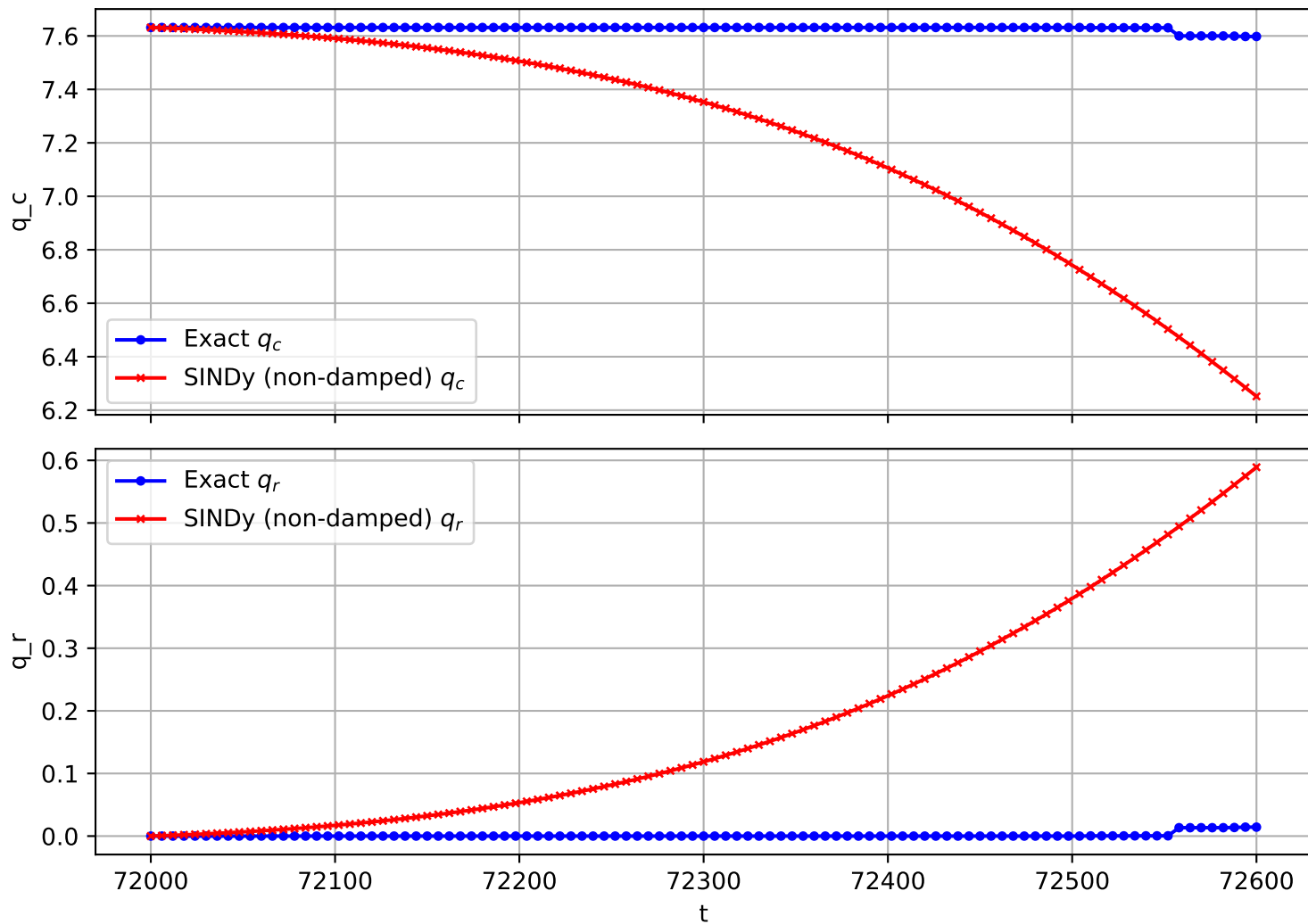
Trajectory 2684 (non-damped)
