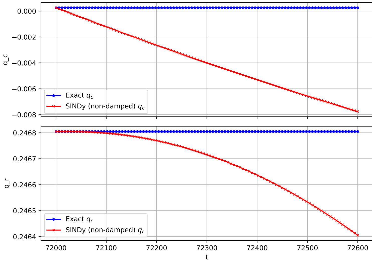
Trajectory 2687 (non-damped)
