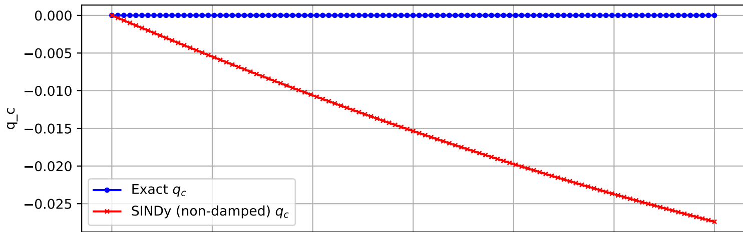
Trajectory 2690 (non-damped)
