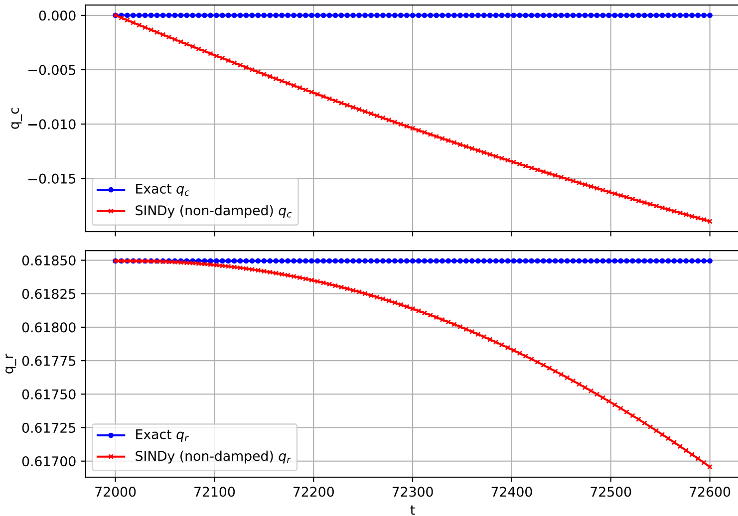
Trajectory 2691 (non-damped)
