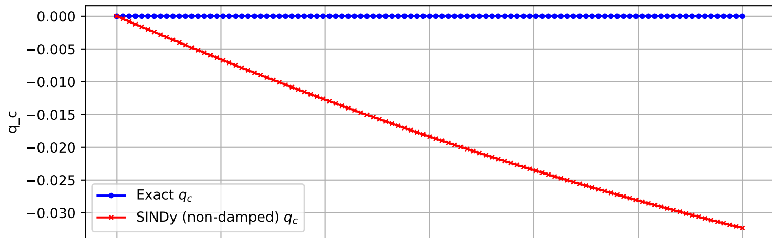
Trajectory 2696 (non-damped)
