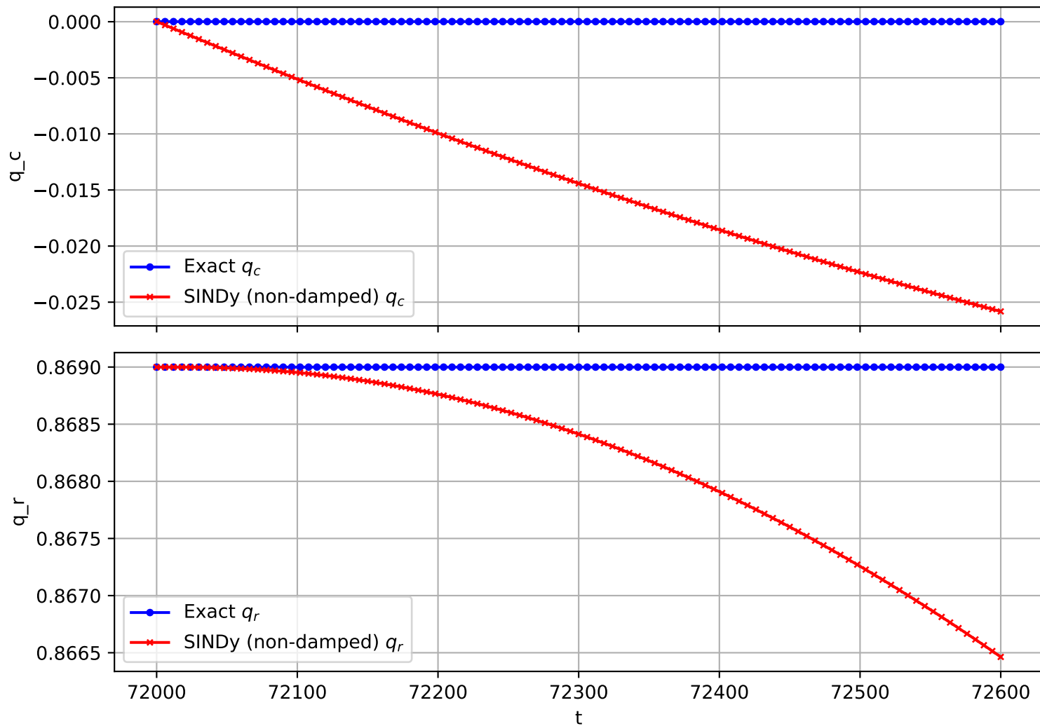
Trajectory 2698 (non-damped)
