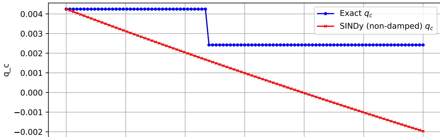
Trajectory 2703 (non-damped)
