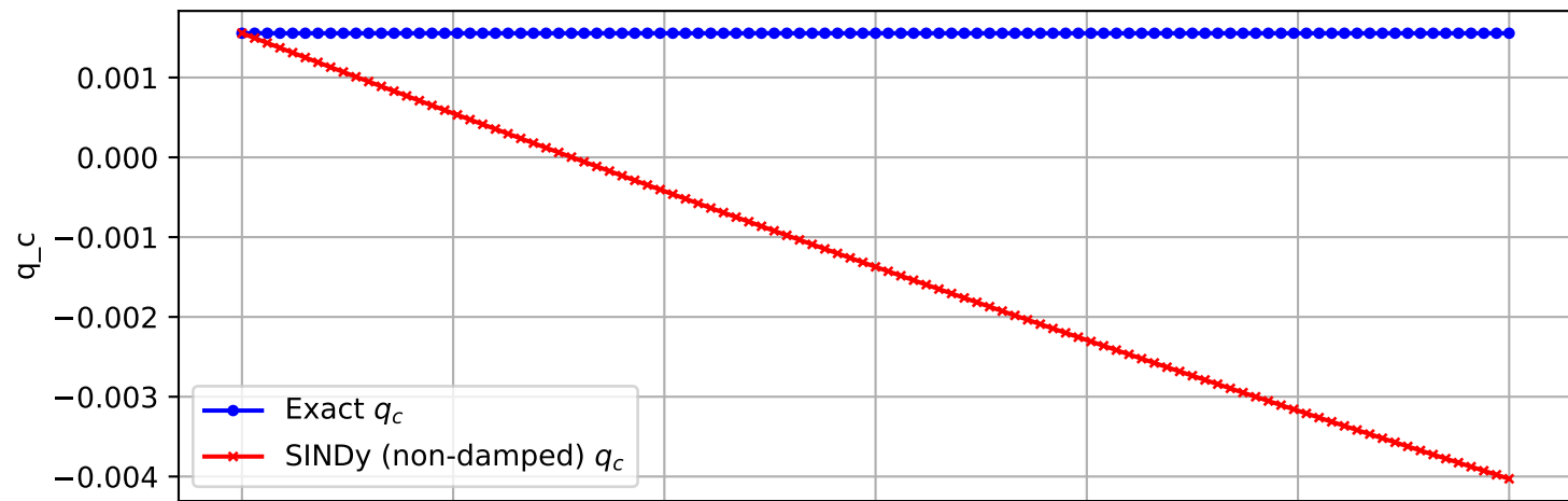
Trajectory 2707 (non-damped)
