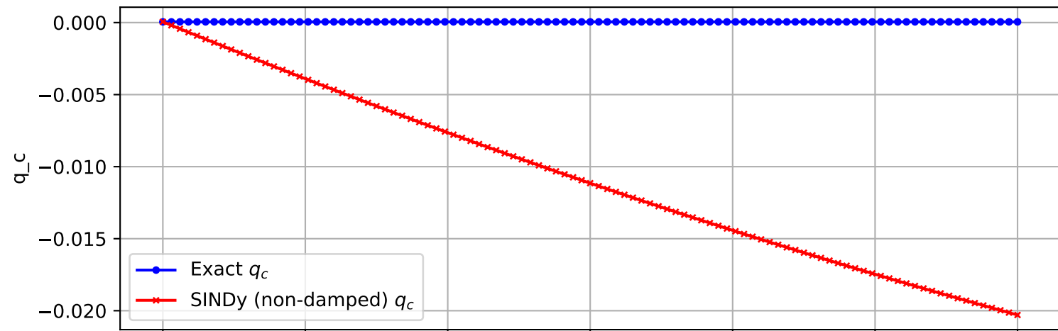
Trajectory 2711 (non-damped)
