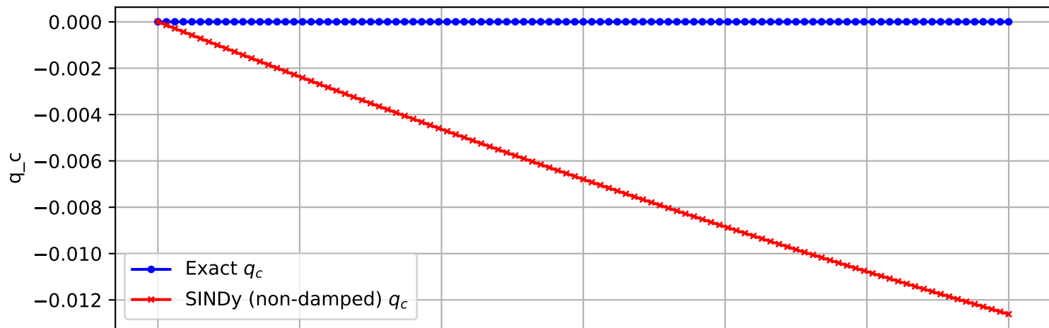
Trajectory 2713 (non-damped)
