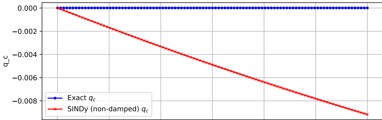
Trajectory 2715 (non-damped)
