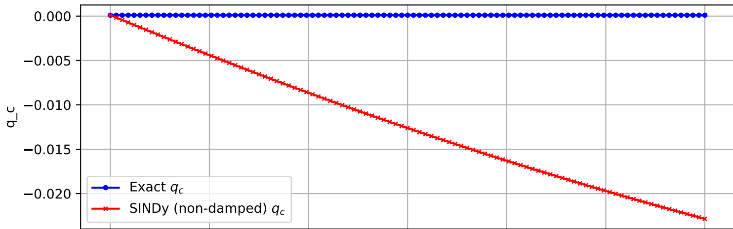
Trajectory 2721 (non-damped)
