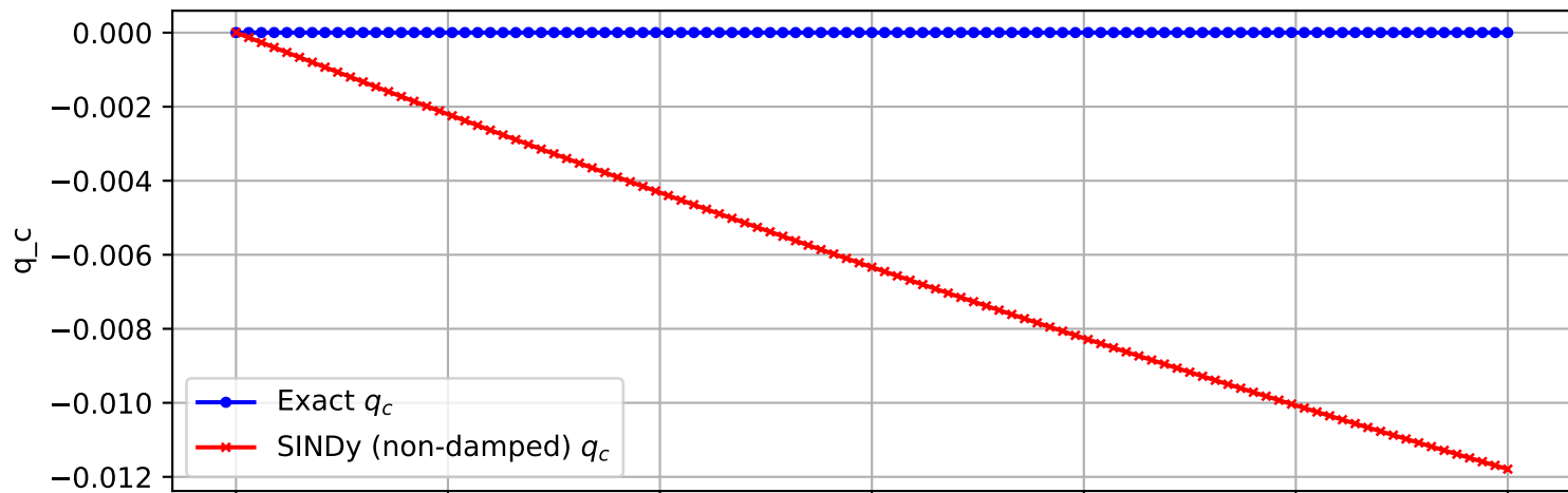
Trajectory 2725 (non-damped)
