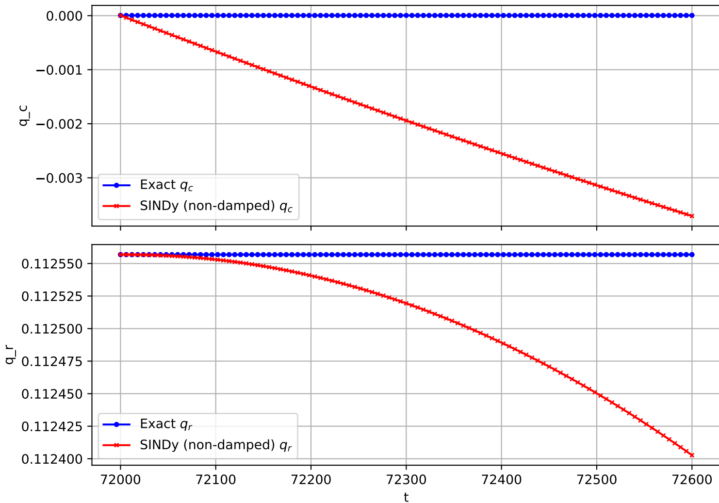
Trajectory 2726 (non-damped)
