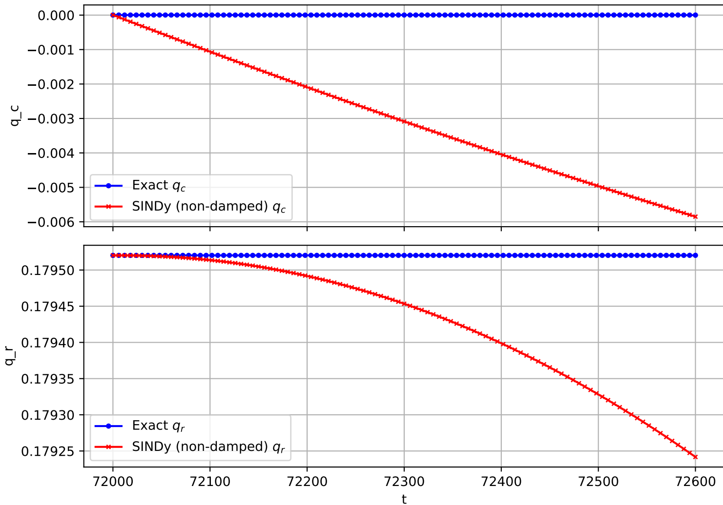
Trajectory 2729 (non-damped)
