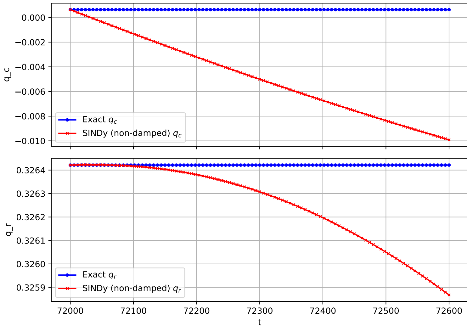
Trajectory 2730 (non-damped)
