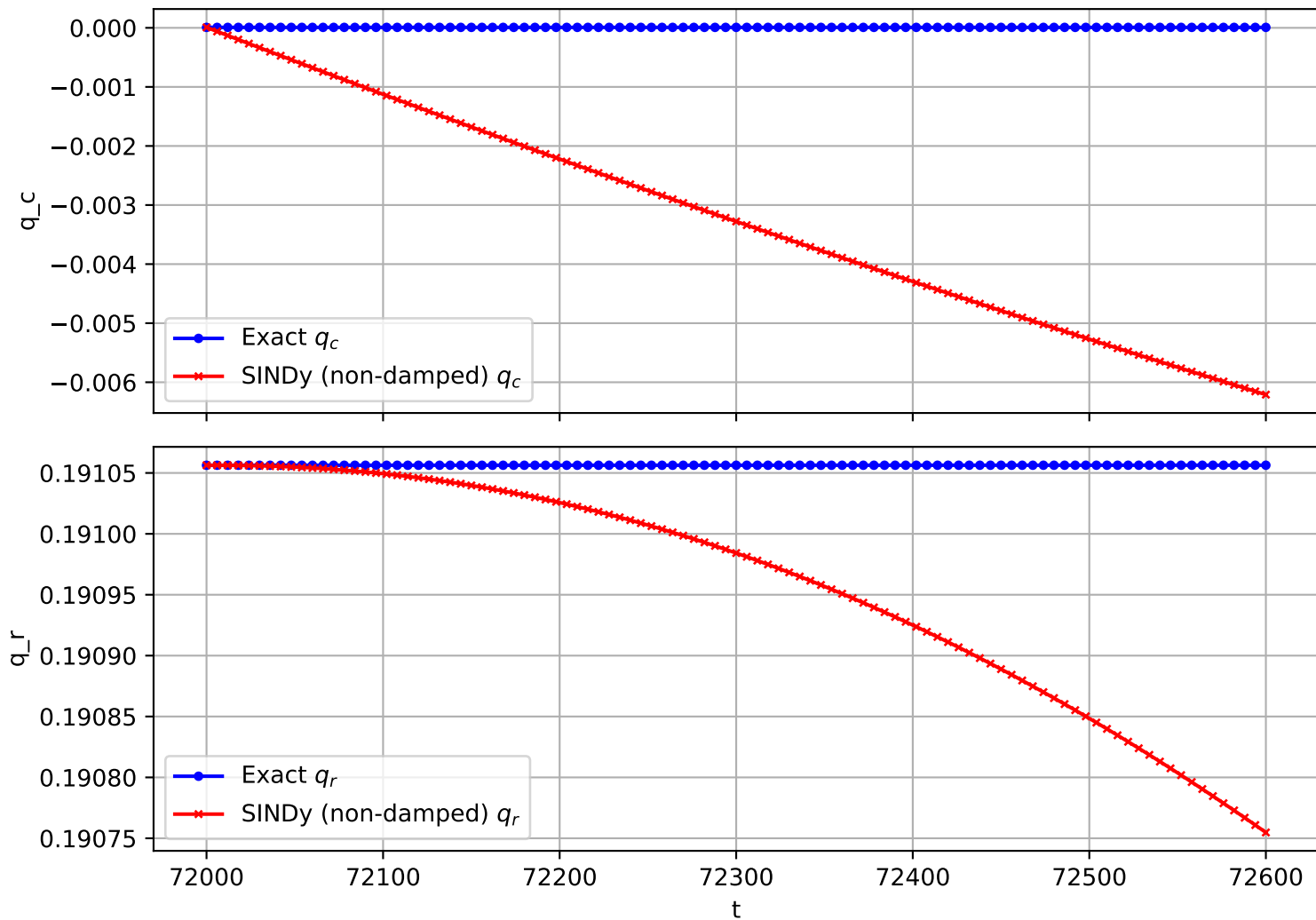
Trajectory 2741 (non-damped)
