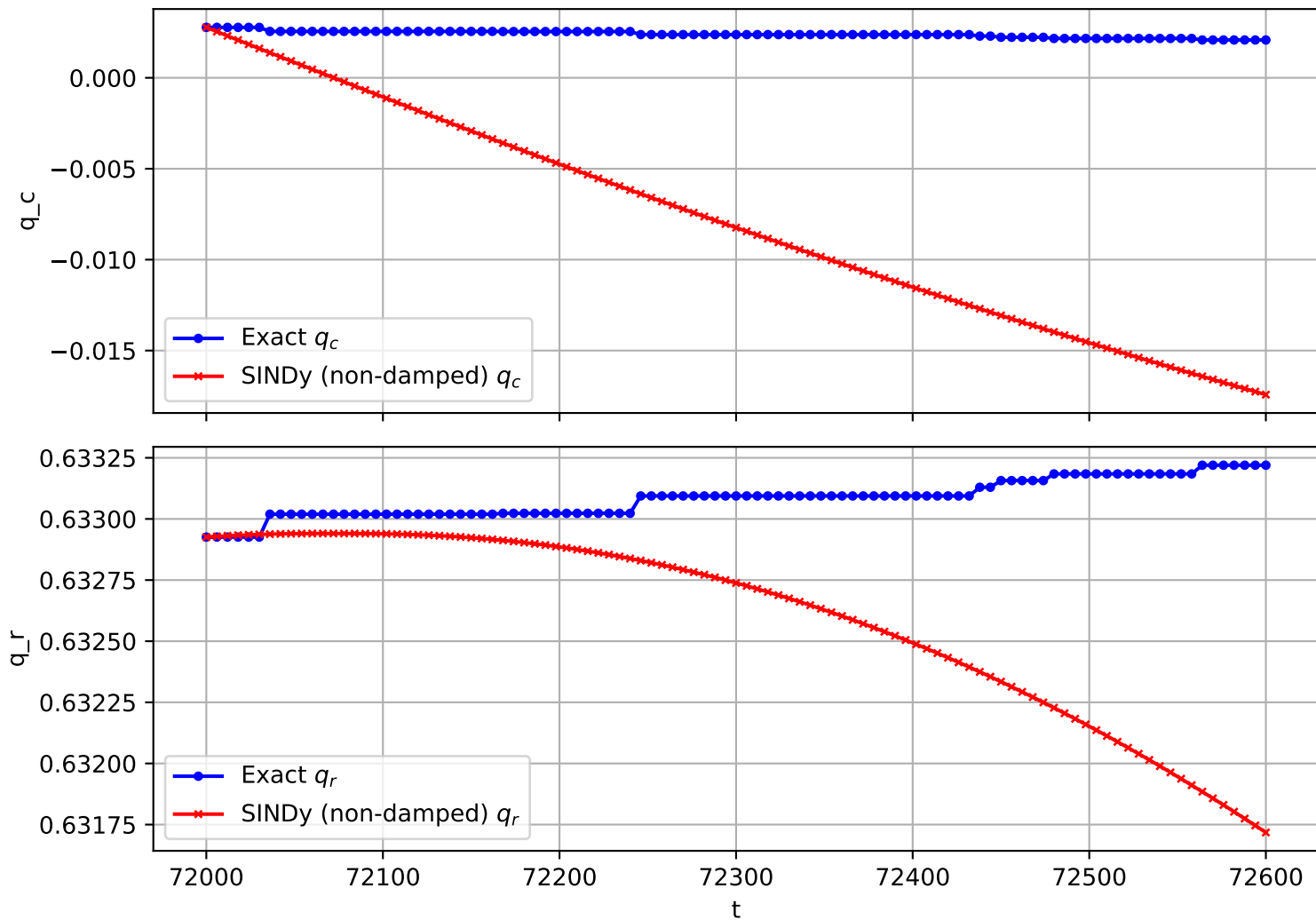
Trajectory 2747 (non-damped)
