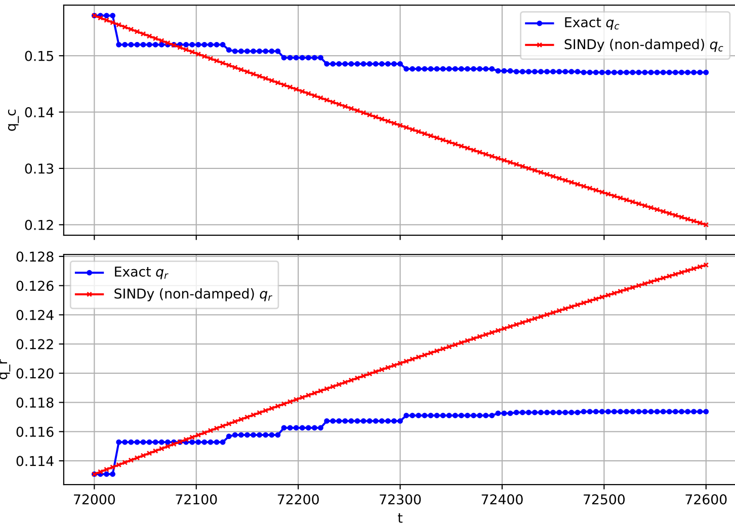
Trajectory 2751 (non-damped)
