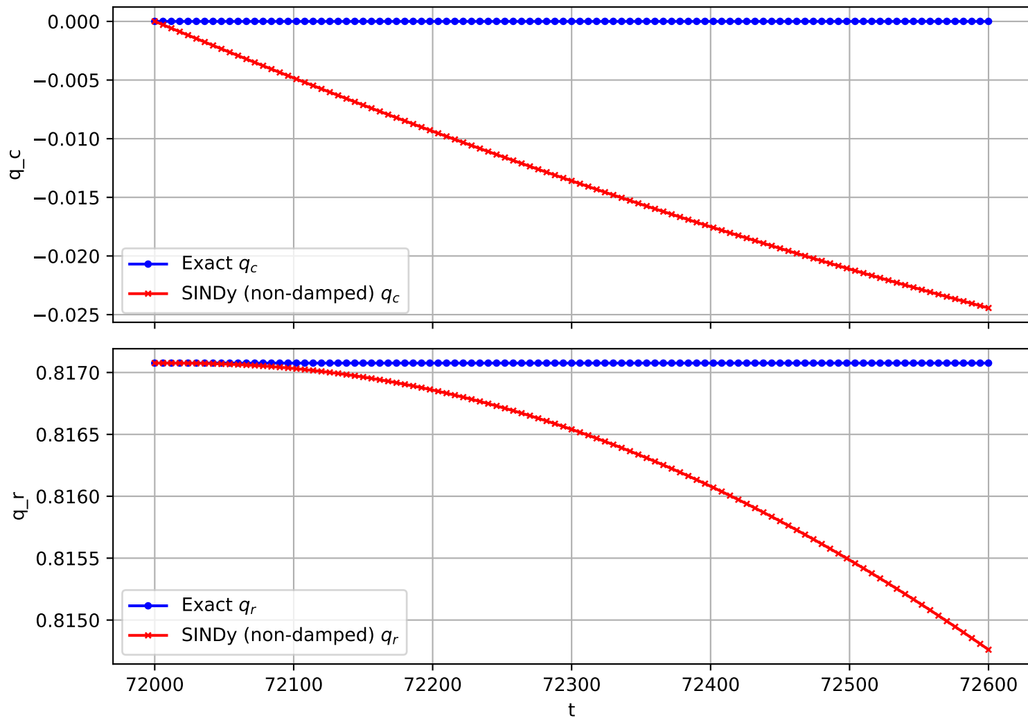
Trajectory 2762 (non-damped)
