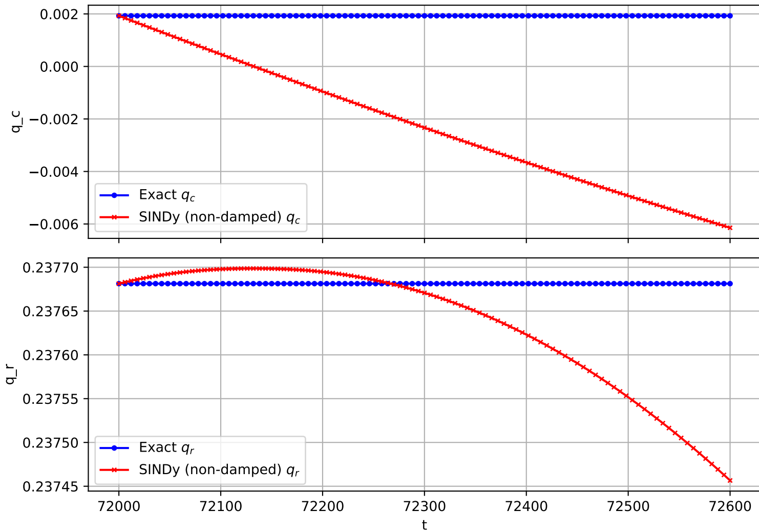
Trajectory 2764 (non-damped)
