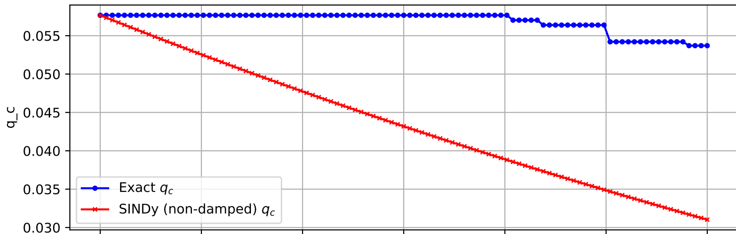
Trajectory 2766 (non-damped)
