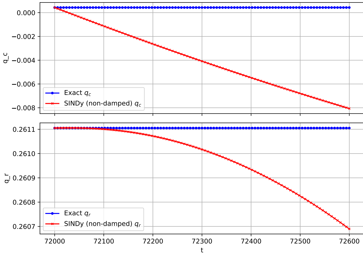
Trajectory 2774 (non-damped)
