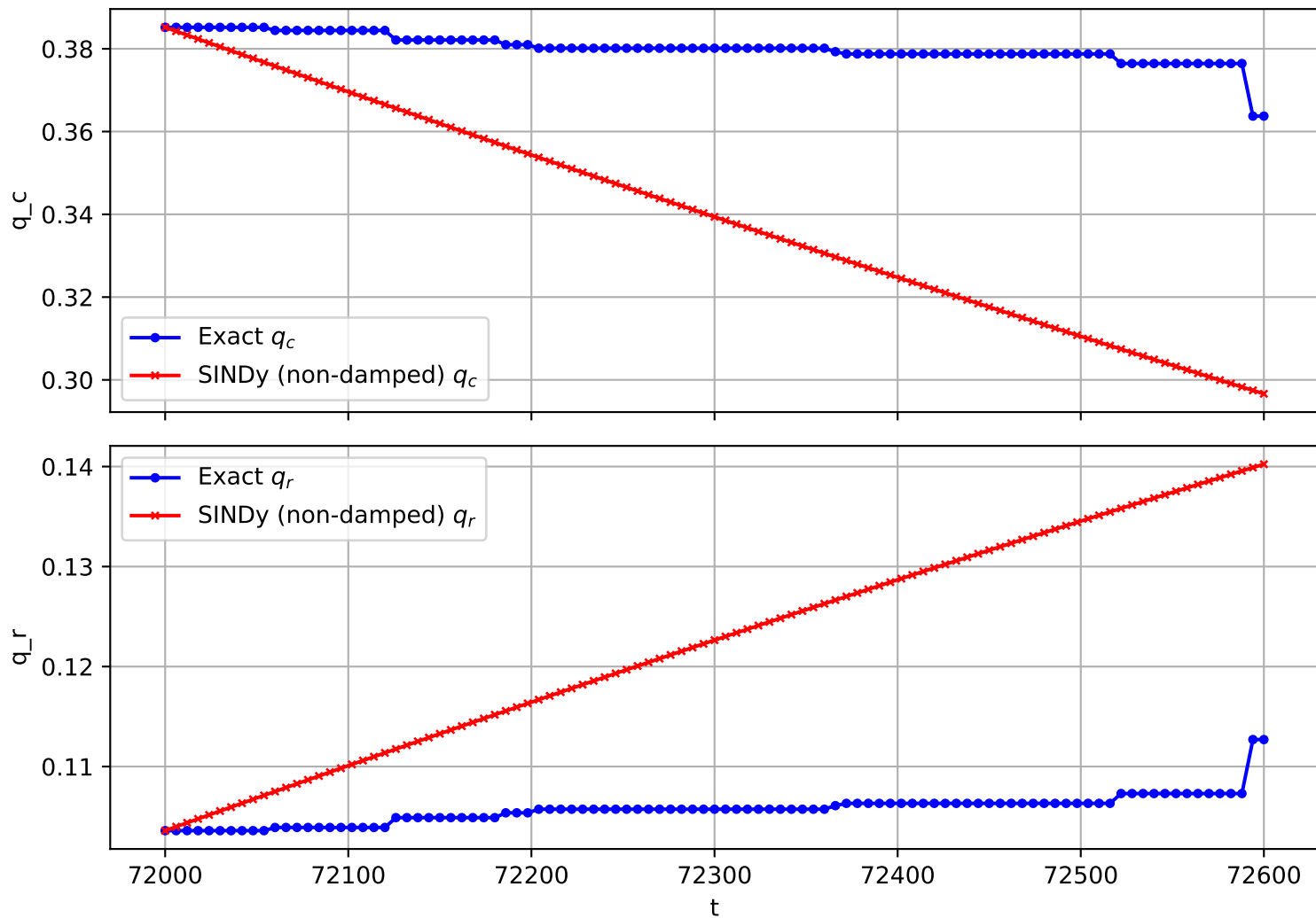
Trajectory 2780 (non-damped)
