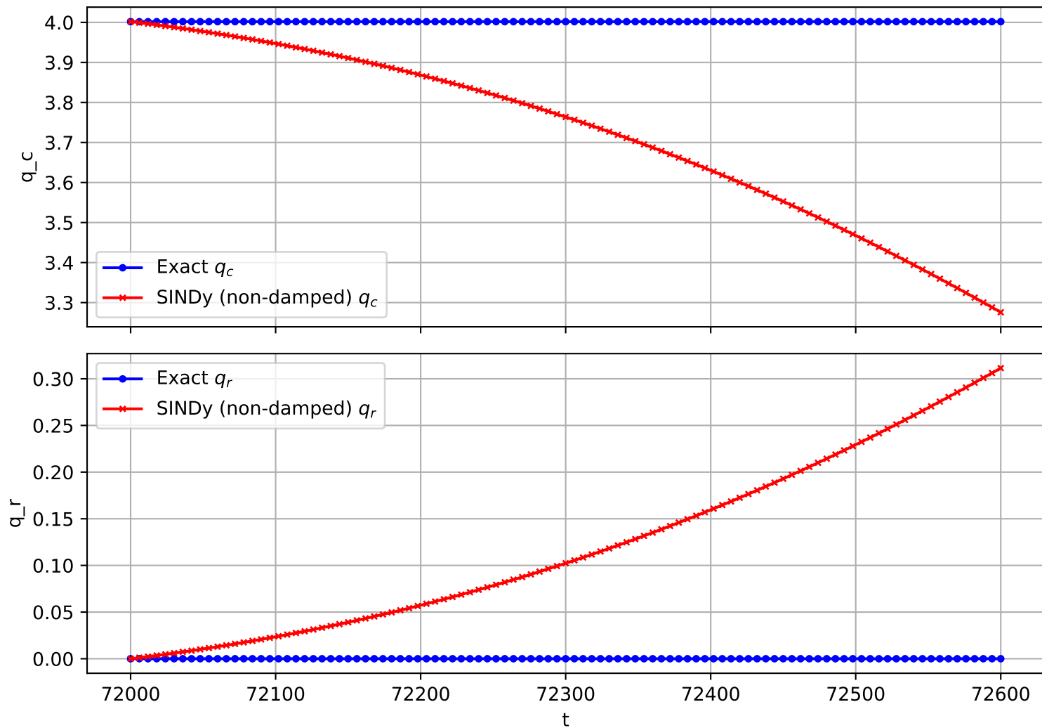
Trajectory 2782 (non-damped)
