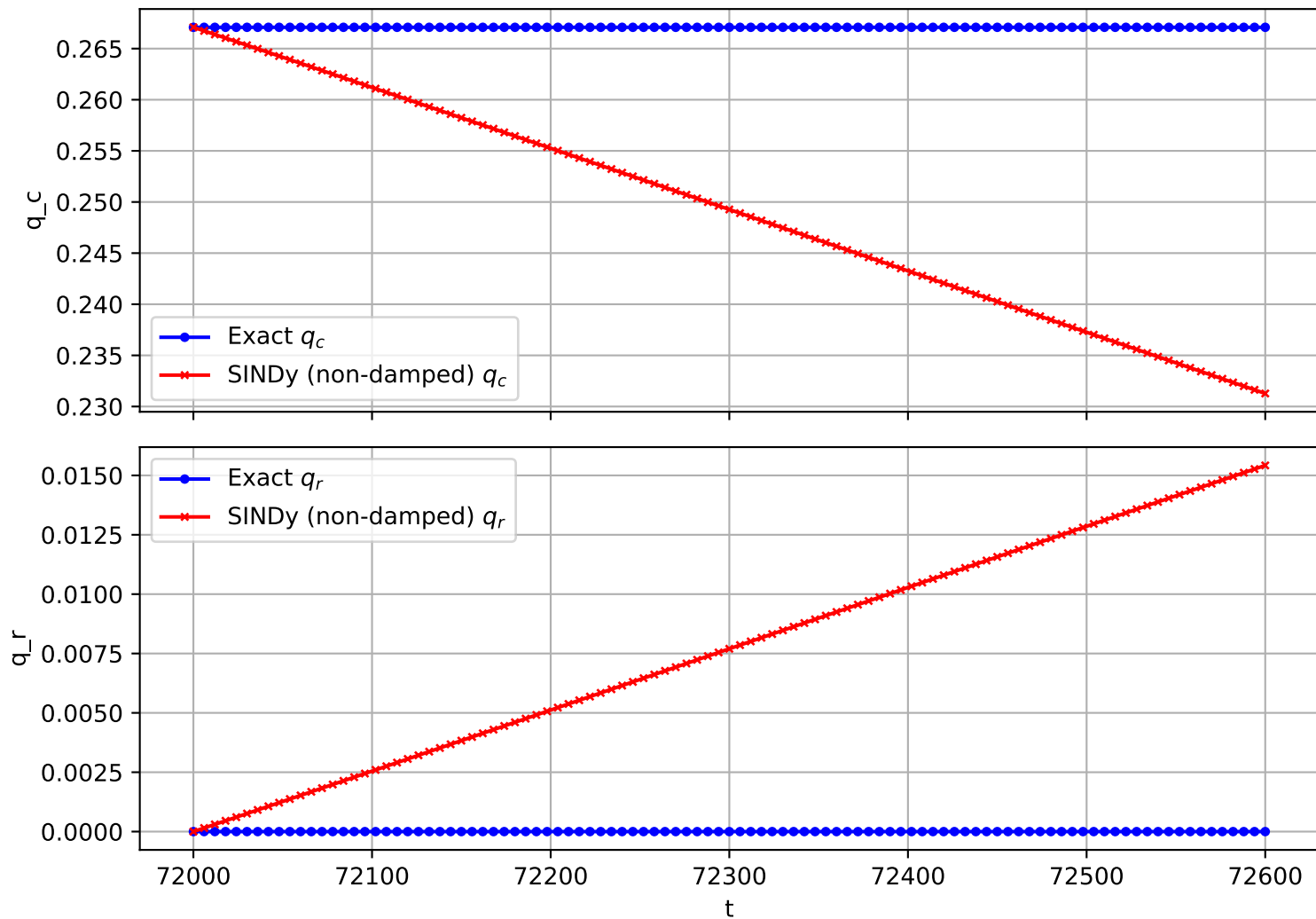
Trajectory 2784 (non-damped)
