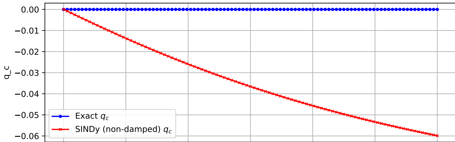
Trajectory 279 (non-damped)
