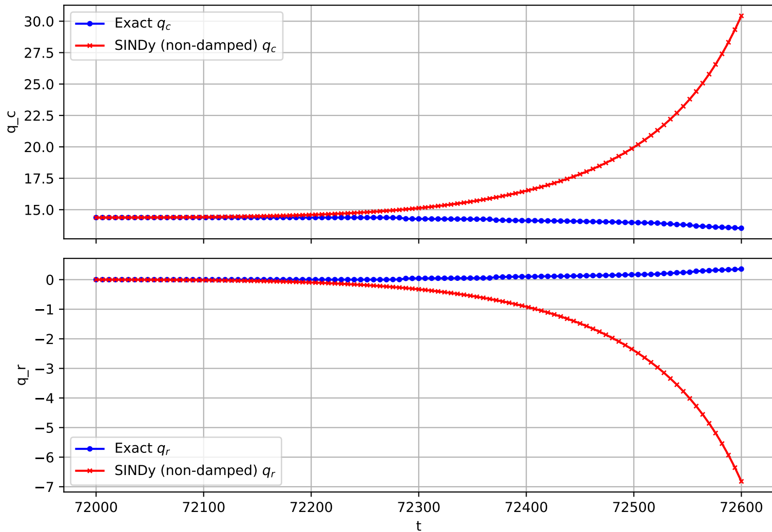
Trajectory 2792 (non-damped)
