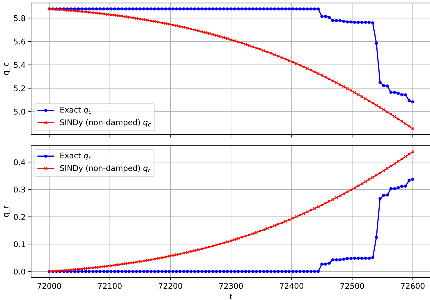
Trajectory 2793 (non-damped)
