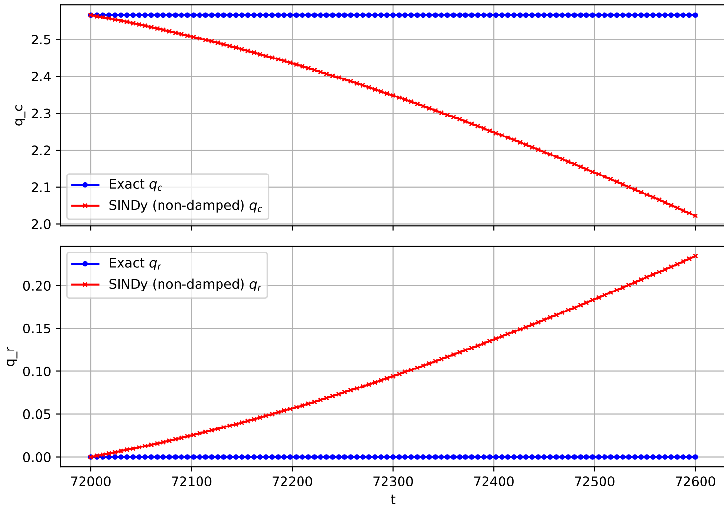
Trajectory 2799 (non-damped)
