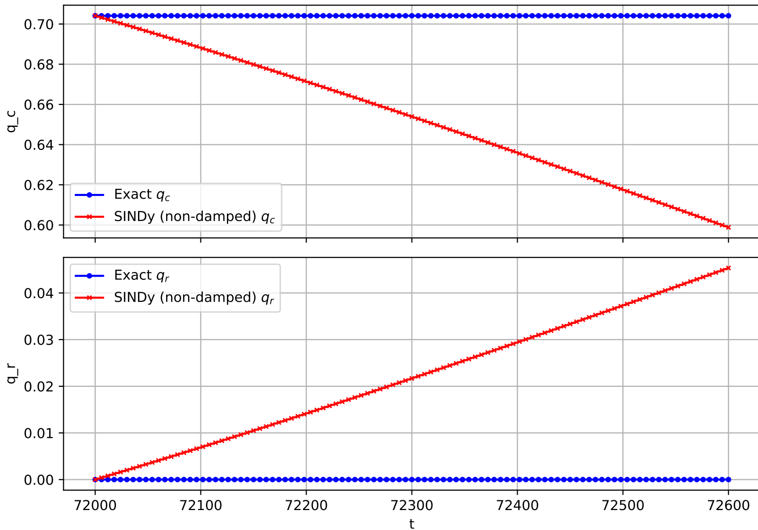
Trajectory 28 (non-damped)
