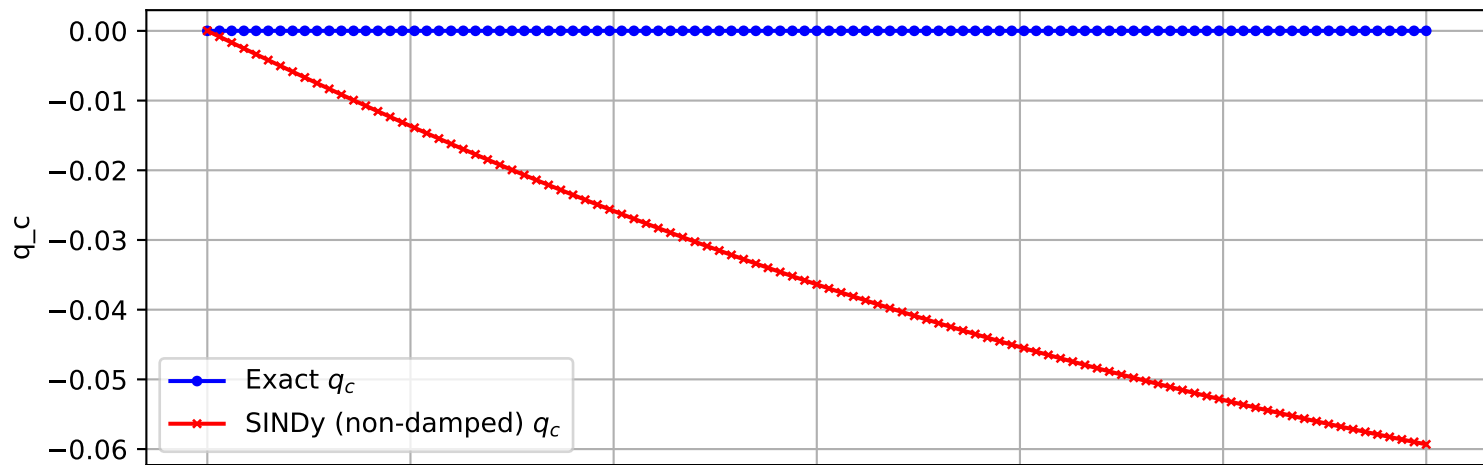
Trajectory 280 (non-damped)
