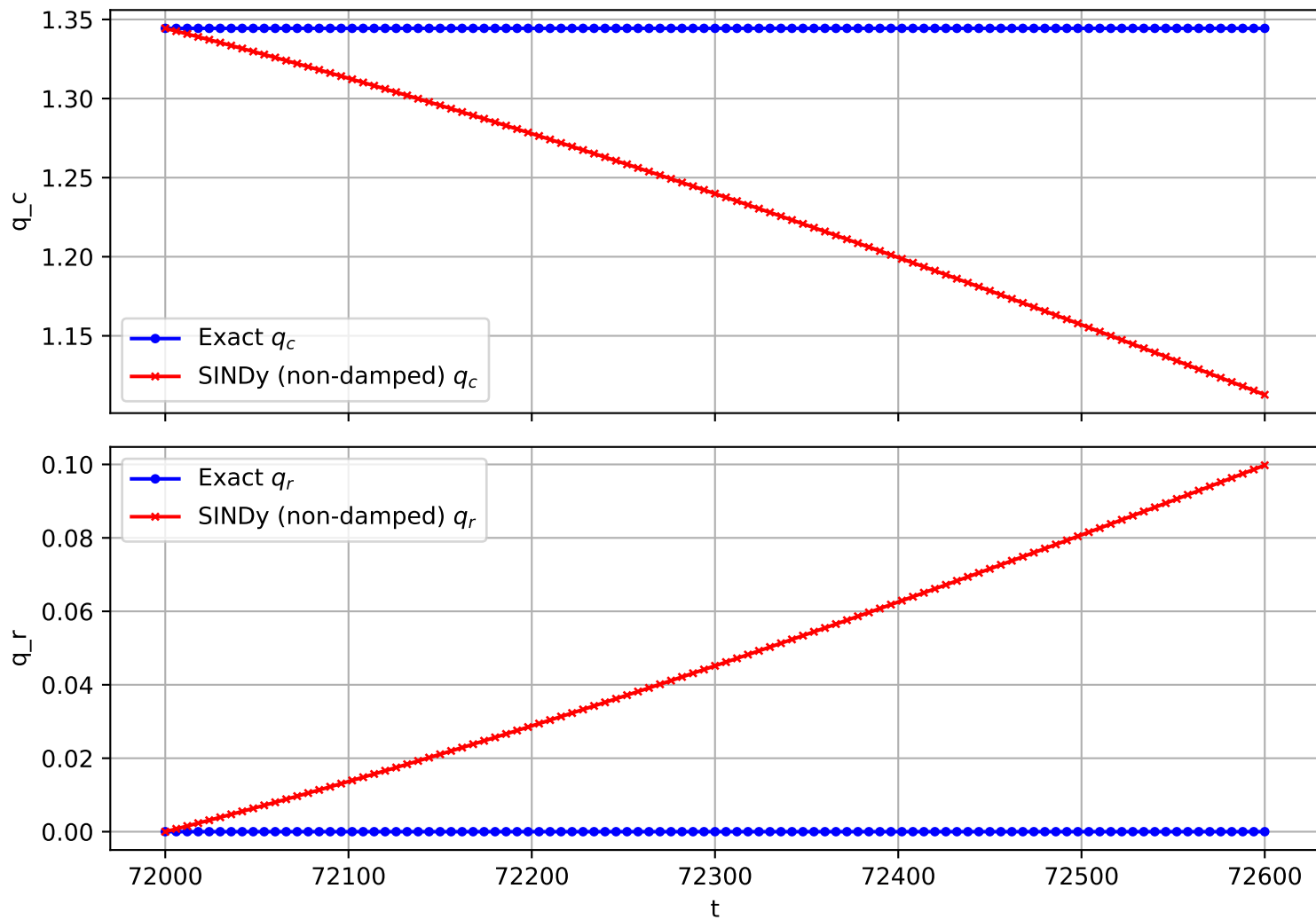
Trajectory 2800 (non-damped)
