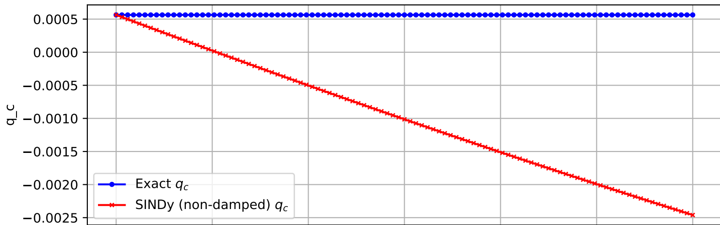
Trajectory 2803 (non-damped)
