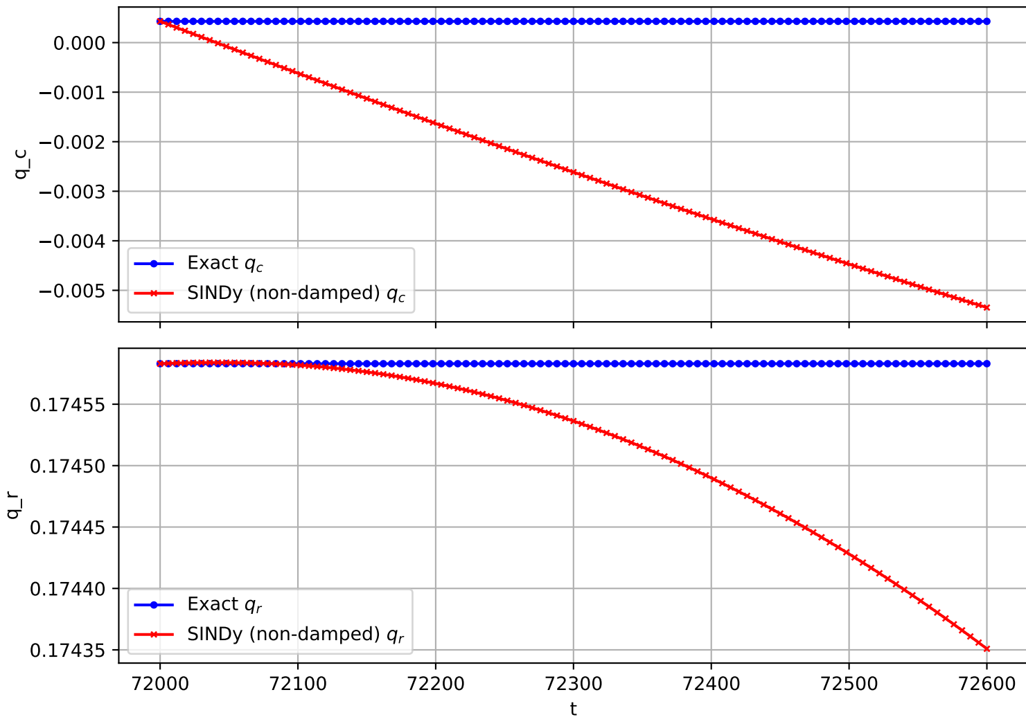
Trajectory 2804 (non-damped)
