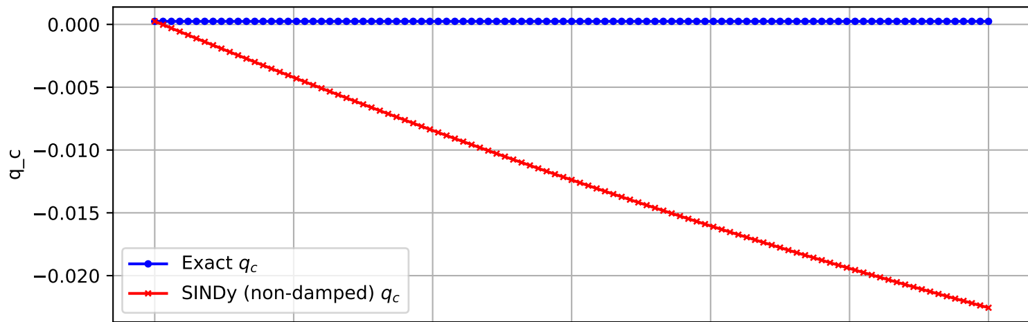
Trajectory 2805 (non-damped)
