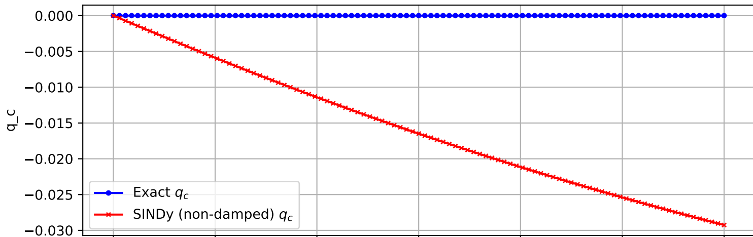
Trajectory 2806 (non-damped)
