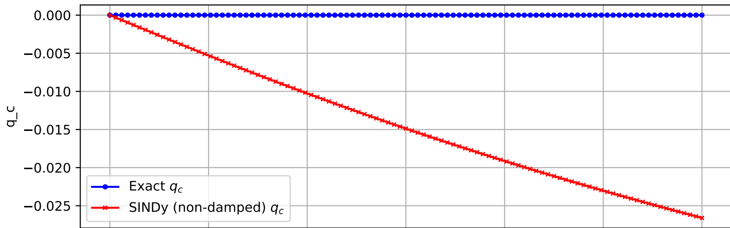
Trajectory 2809 (non-damped)
