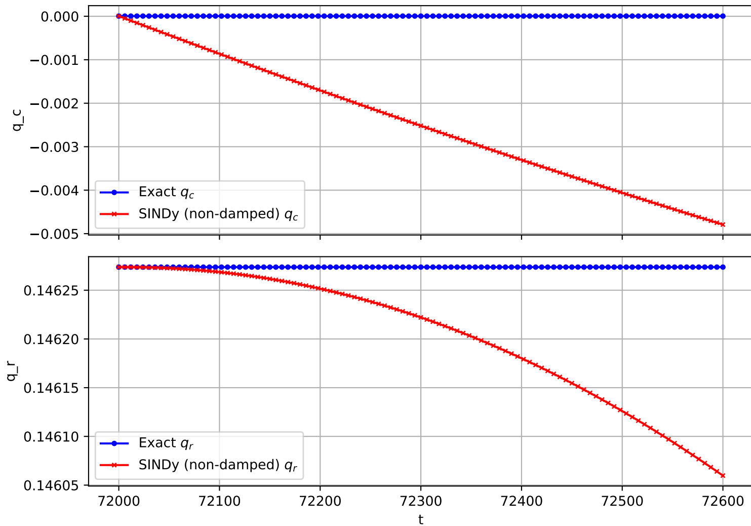
Trajectory 2812 (non-damped)
