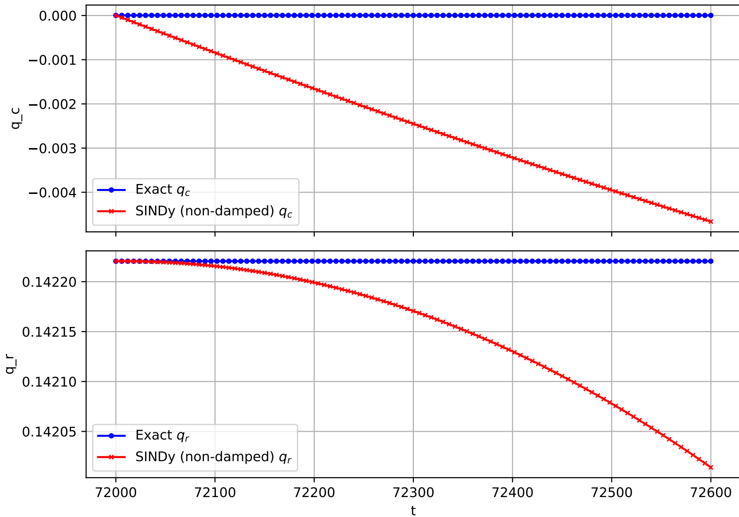
Trajectory 2823 (non-damped)
