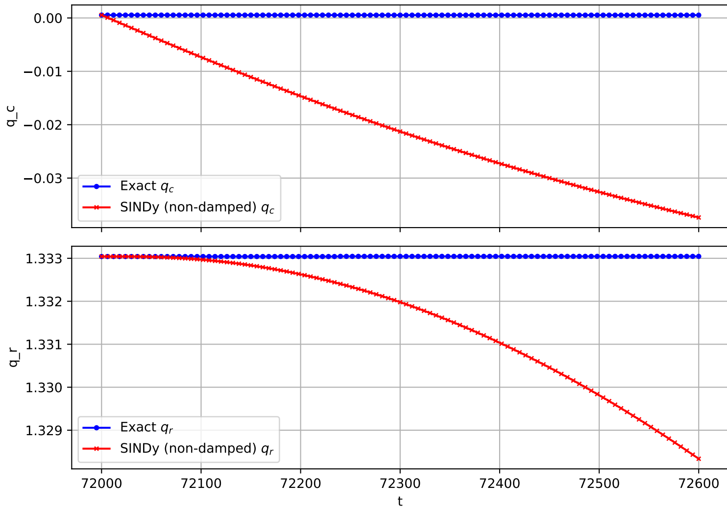
Trajectory 2828 (non-damped)
