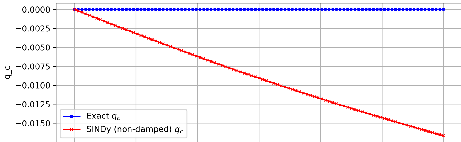
Trajectory 2833 (non-damped)
