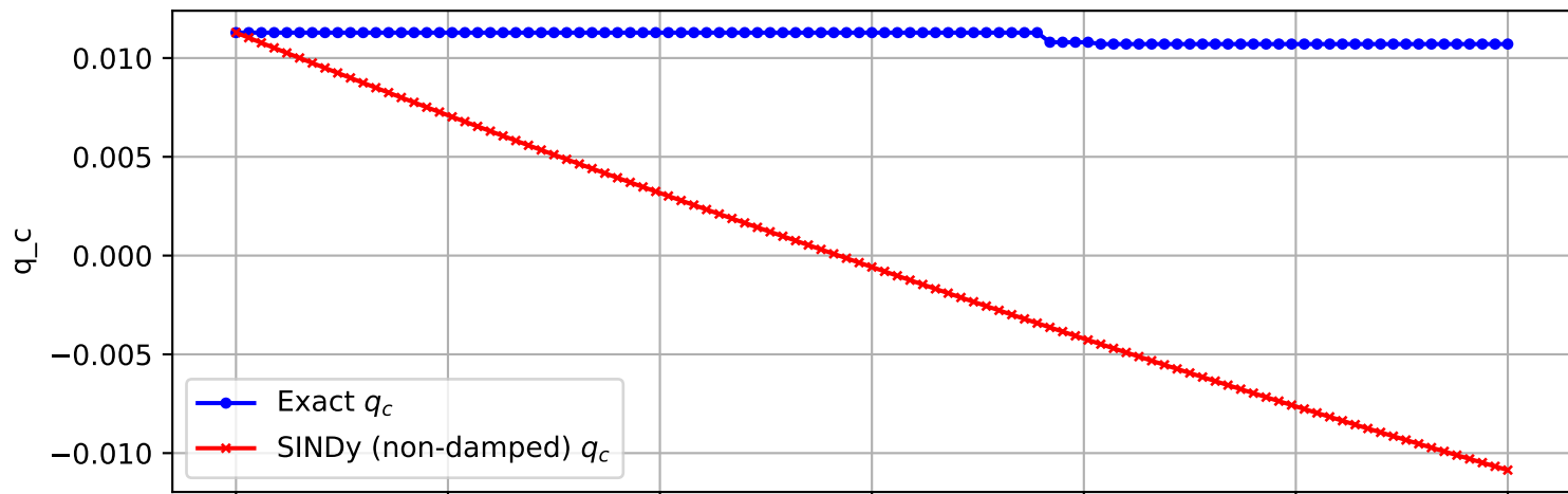
Trajectory 2839 (non-damped)
