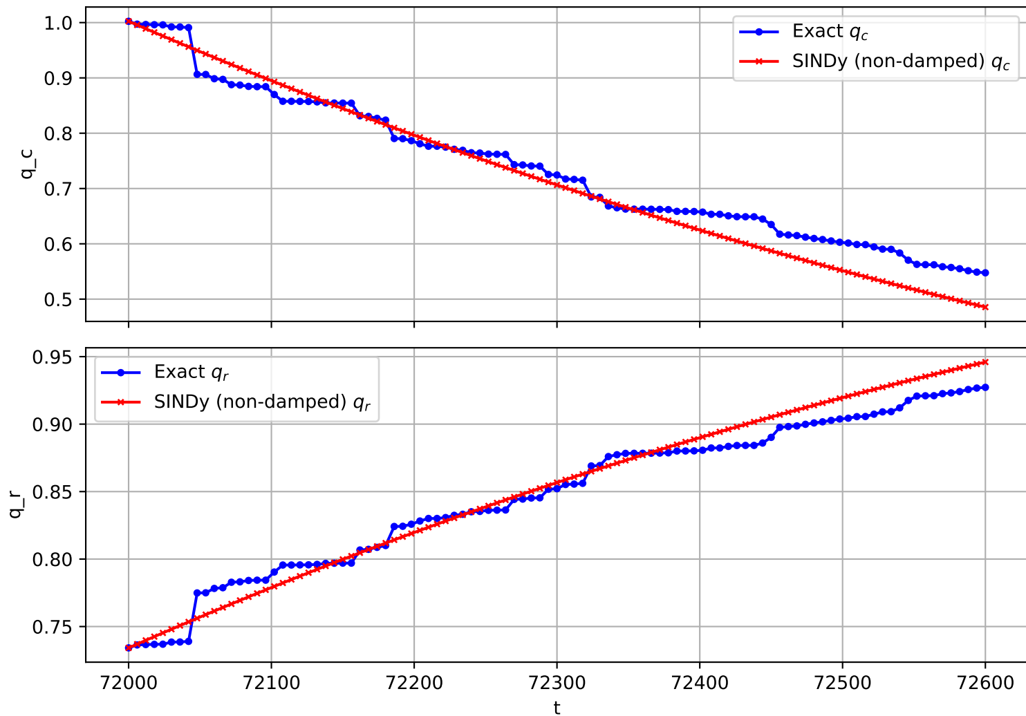
Trajectory 2841 (non-damped)
