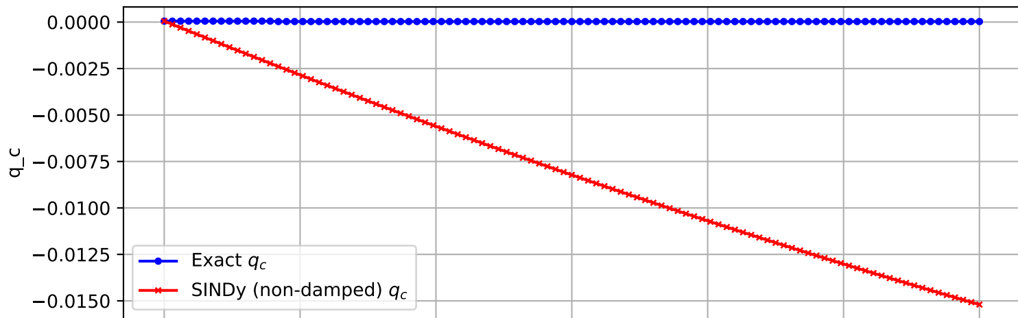
Trajectory 2844 (non-damped)
